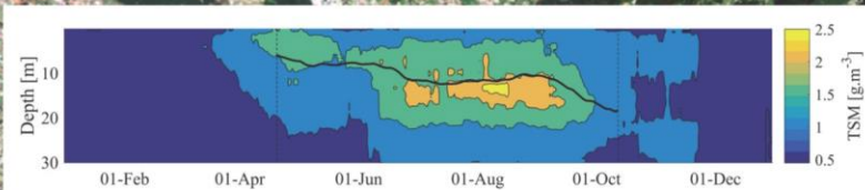
Fig. 1: Vertical TSM gradients at SHL2 and thermocline depth (black line), 2002-2015 averaged (Nouchi et al., 2018).
